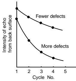
FIGURE G.6 Attenuation of ultrasonic wave upon traveling through the material. One cycle means traveling from the front surface to the back surface and then to the front surface.
