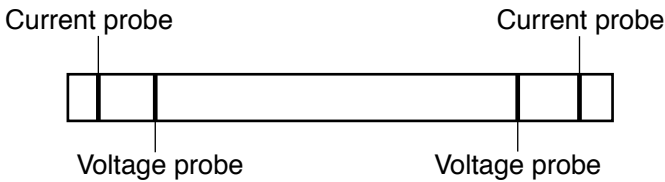
FIGURE C.2 The four-probe method of resistance/impedance measurement.
