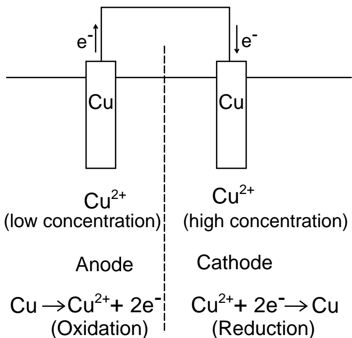
FIGURE H.3 Concentration cell with Cu electrodes, a low Cu 2+ concentration at the anode side, and a high Cu 2+ concentration at the cathode side.
