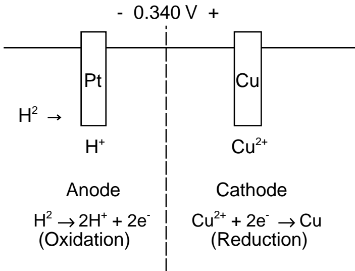
FIGURE H.8 A cell with copper as the cathode and the hydrogen half-cell as the anode under open-circuit condition. The open-circuit voltage is 0.340 V — positive at the cathode.
