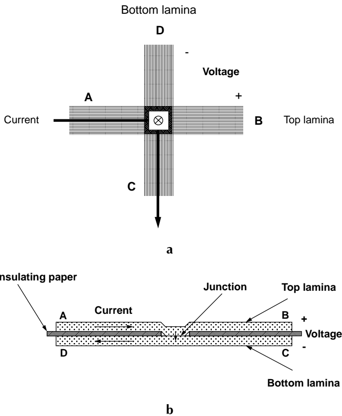
FIGURE 6.1 Specimen configuration for measurement of the contact electrical resistivity between laminae: (a) cross-ply laminae, (b) unidirectional laminae.
