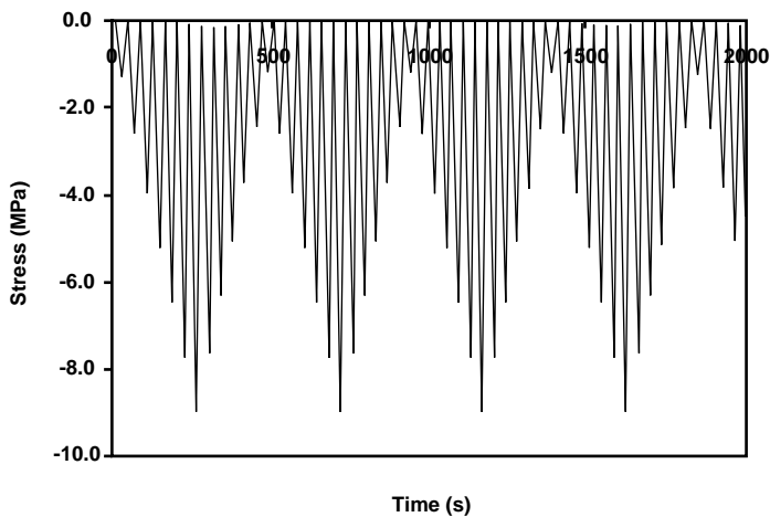
FIGURE 5.10 Fractional change in resistance (a), strain (a), and stress (b) during repeated compressive loading at increasing and decreasing stress amplitudes, the highest of which was >90\% of the compressive strength, for carbon fiber concrete at 28 days of curing.
