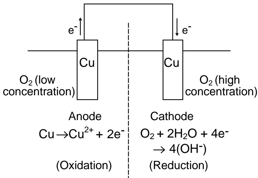
FIGURE H.4 Oxygen concentration cell with Cu electrodes, a low O 2 concentration at the anode side, and a high O 2 concentration at the cathode side.
