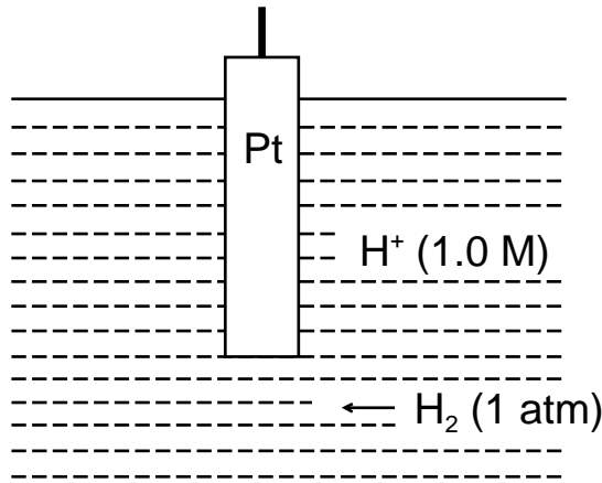
FIGURE H.7 The standard hydrogen reference half-cell.
