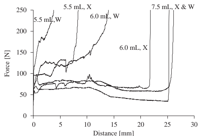
Fig. 5. Typical extrusion curves obtained with various amounts of mixing liquid (5.5, 6.0 and 7.5 ml) and various liquids (water (W) or 0.2% xanthan solution (X)).
