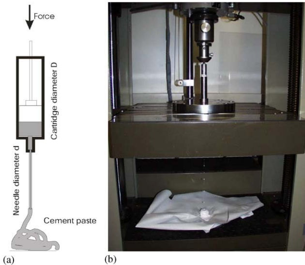
Fig. 4. Experimental setup showing (a) a scheme of the mixing and injection device, and (b) the paste falling down.
