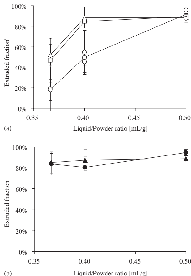
Fig. 6. Extruded fraction of the paste as a function of the LPR and the composition of the mixing liquid. (a) Unmilled \beta -TCP powder: (○) water; (Δ) PAA 1% solution; (□) xanthan 0.2% solution; and (b) milled \beta -TCP powder: (●) water; (▲) PAA 1% solution. The error bars indicate the 95% confidence interval on the mean.
