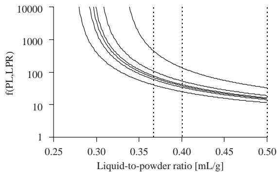
Fig. 1. Variation of f(\text{PL}; \text{LPR}) as a function of the liquid-to-powder ratio, LPR, and the plastic limit, PL. Six curves are represented corresponding to the six pastes tested in this study. From bottom to top: (i) milled \beta -TCP, PAA solution; (ii) Unmilled \beta -TCP, PAA solution; (iii) milled \beta -TCP, xanthan solution; (iv) milled \beta -TCP, water; (v) unmilled \beta -TCP, xanthan solution; (vi) unmilled \beta -TCP, water.
