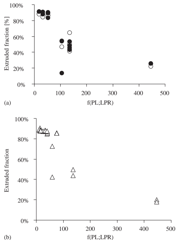
Fig. 7. Relationship between the extruded fraction and the function f(\text{PL}, \text{LPR}) . (a) Results obtained in the first and second factorial design; (○) gauge 10 and (●) gauge 14. (b) Results obtained in the third factorial design.
