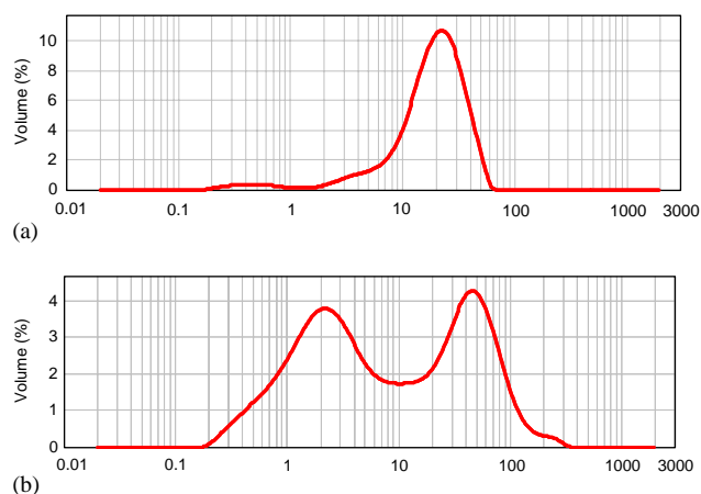
Fig. 3. Particle size volume distribution of (a) unmilled and (b) milled \beta -TCP powder as measured by laser granulometry in water. The size (x-axis) is given in micrometers. A similar result is obtained in isopropanol.
