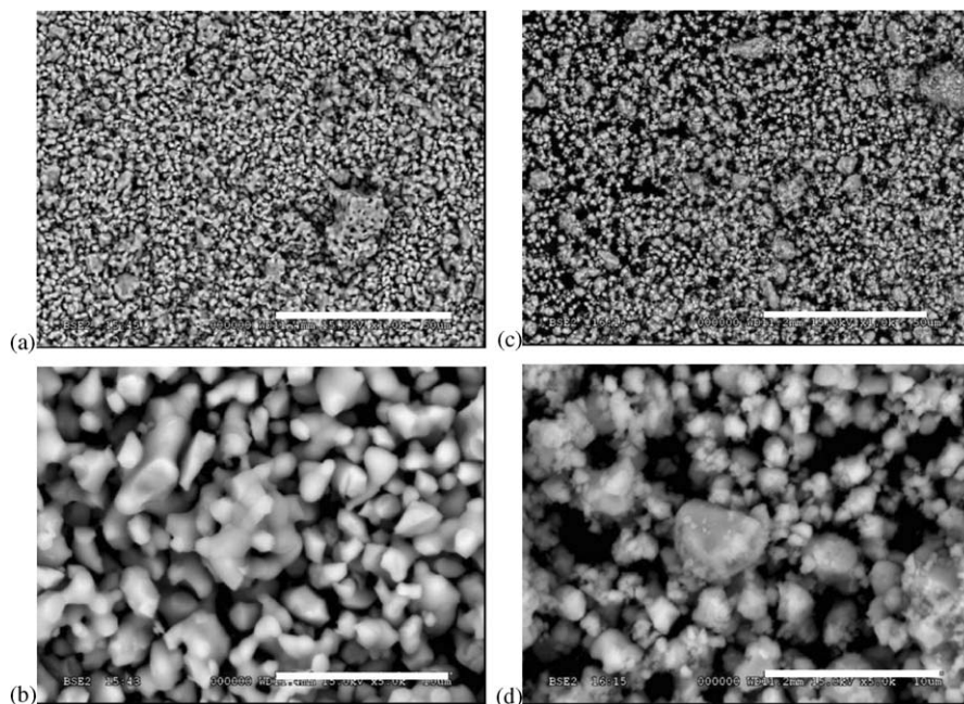
Fig. 2. SEM photos of (a, b) unmilled powder and (c, d) milled powder. The error bars (white line) correspond to a size of (a, c) 50 \mu\text{m} and (b, d) 10 \mu\text{m} .
