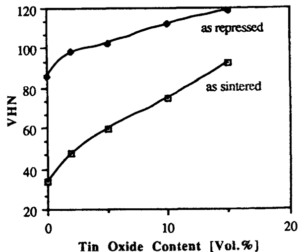
Fig. 7 Hardness as sintered and as cold rolled at different tin oxide volume loading.
