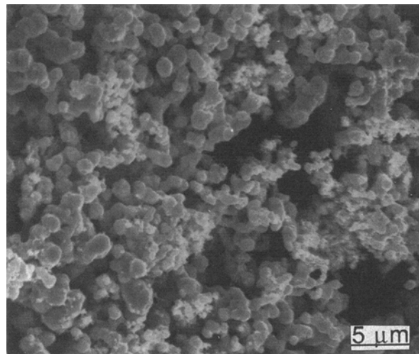
Fig. 3 Scanning electron micrograph of silver-15 vol.% tin oxide composite powders.
